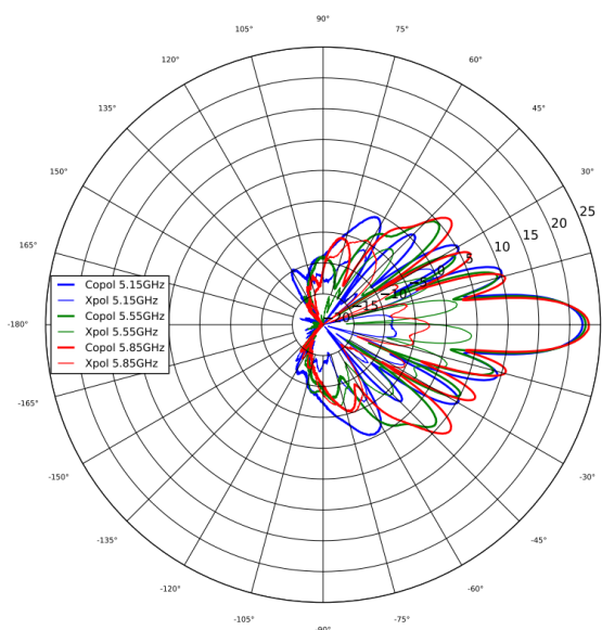
5 GHz Azimuth
