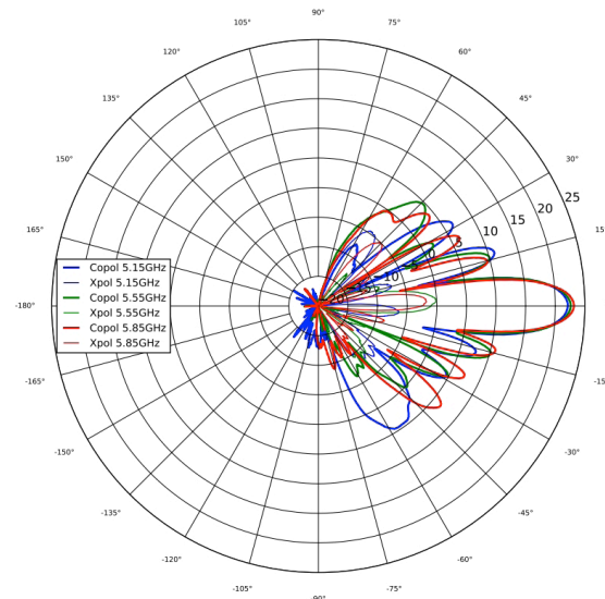
5 GHz Elevation
