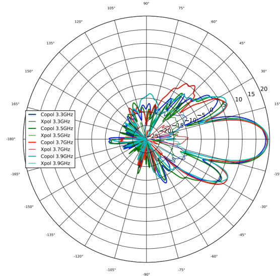
3 GHz Elevation
