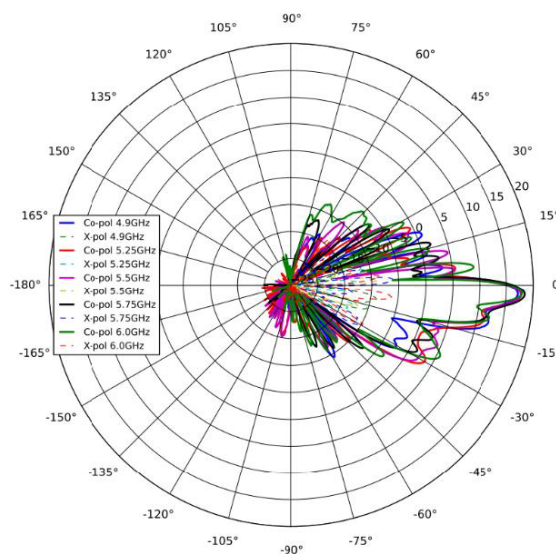
5 GHz Elevation
