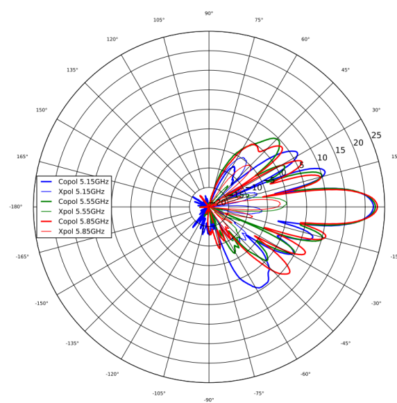
5 GHz Elevation
